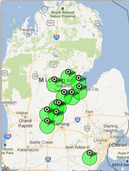
RTK Base Stations
